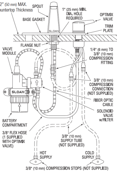
EBF-85-4 Faucet
