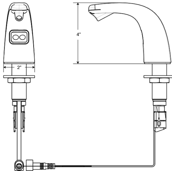
ESD-600 Soap Dispenser
