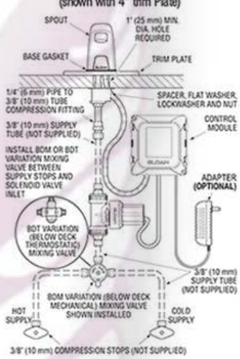
EBF-615 Faucet with BDM and BDT Variation Mixing Valves for Hot and Cold Water Supply (shown with 4" trim Plate)
