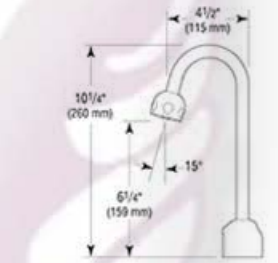
EBF-750-H with Standard Spout and Shower Spray Head †
