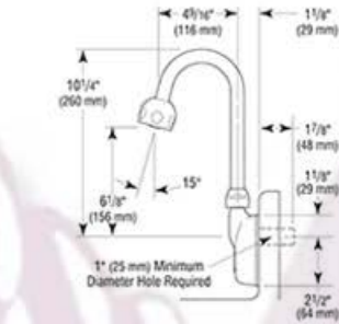
EBF-550-S-H with Surgical Bend Spout and Shower Spray Head †
