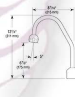
EBF-750-S-H with Surgical Bend Spout and Shower Spray Head †
