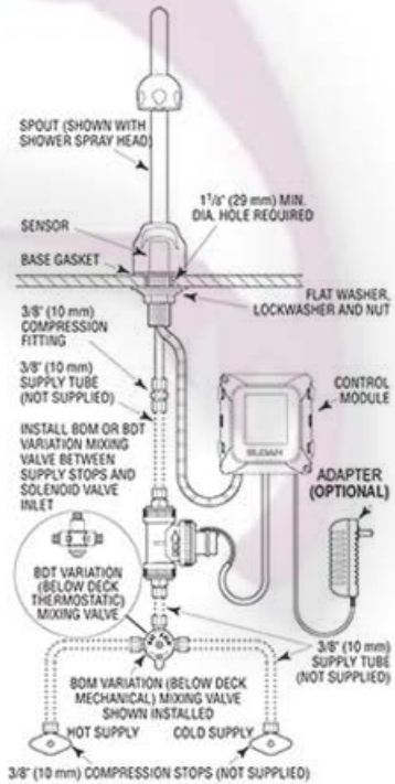
EBF-750 Faucet with BDM and BDT Variation Mixing Valves for Hot and Cold Water Supply †
