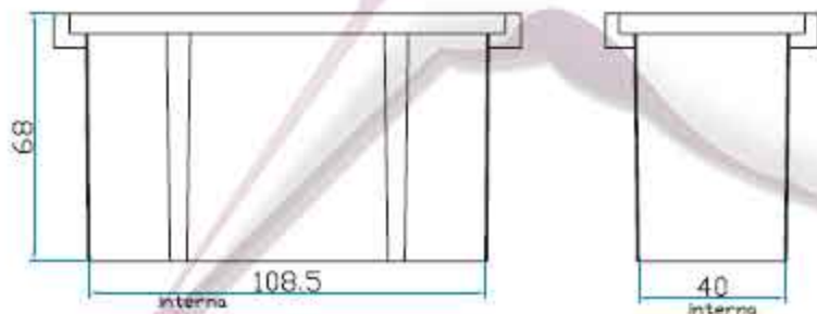
VISTA FRONTAL
