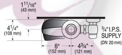
CENTERLINE OF FIXTURE
