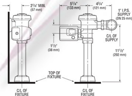
Includes EBV-89-A Side Mount Operator
